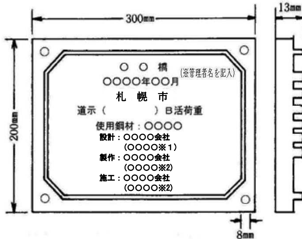
板厚8mm 字厚5mm 計13mm
