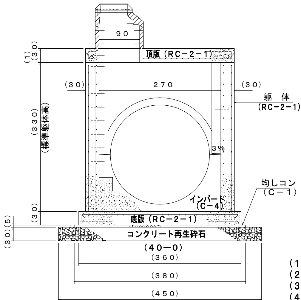
&lt;断面図&gt; S = 1/50
