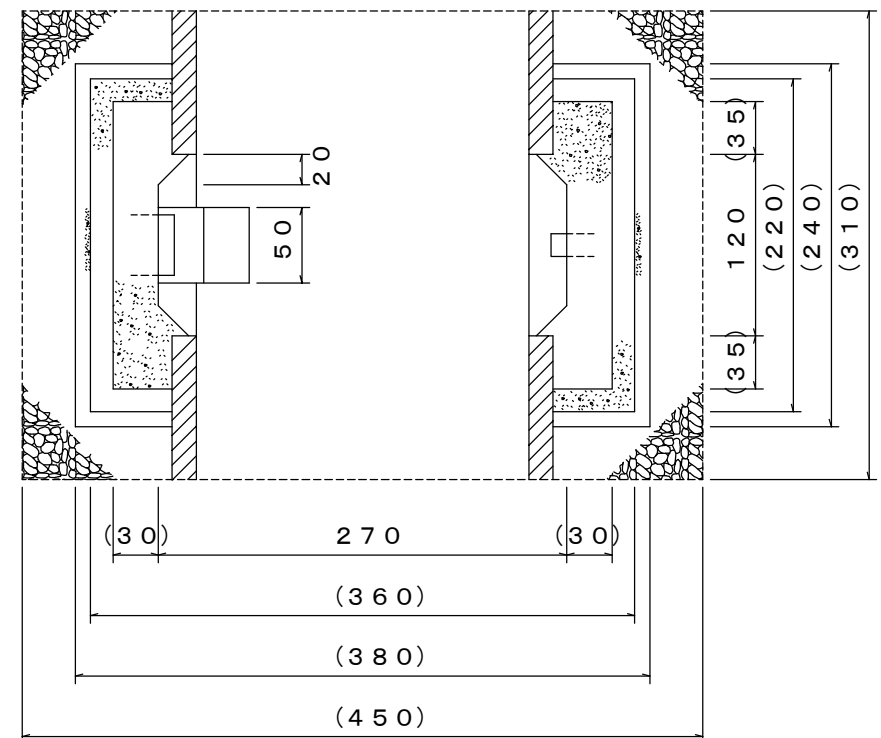
&lt;平面図&gt; S = 1/50
