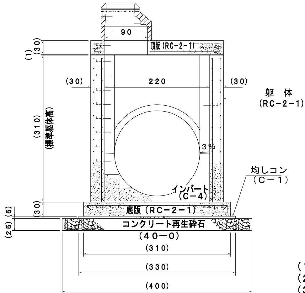
&lt;断面図&gt; S = 1/50
