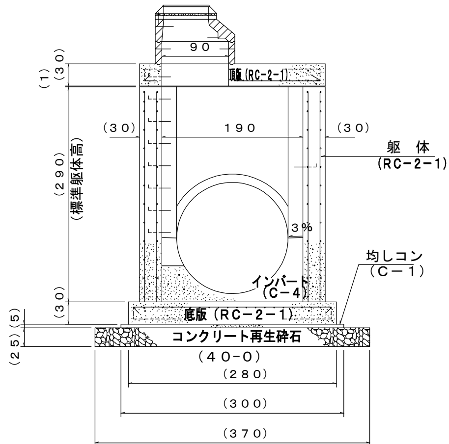
&lt;断面図&gt; S = 1/50
