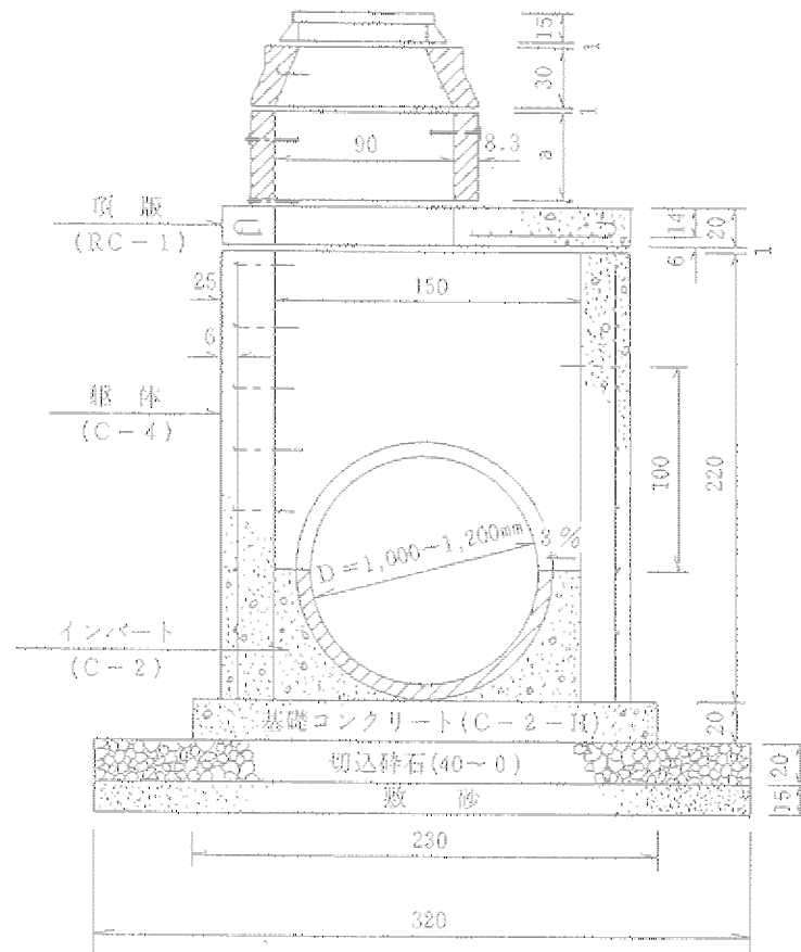
＜断面図＞ S=1/40
